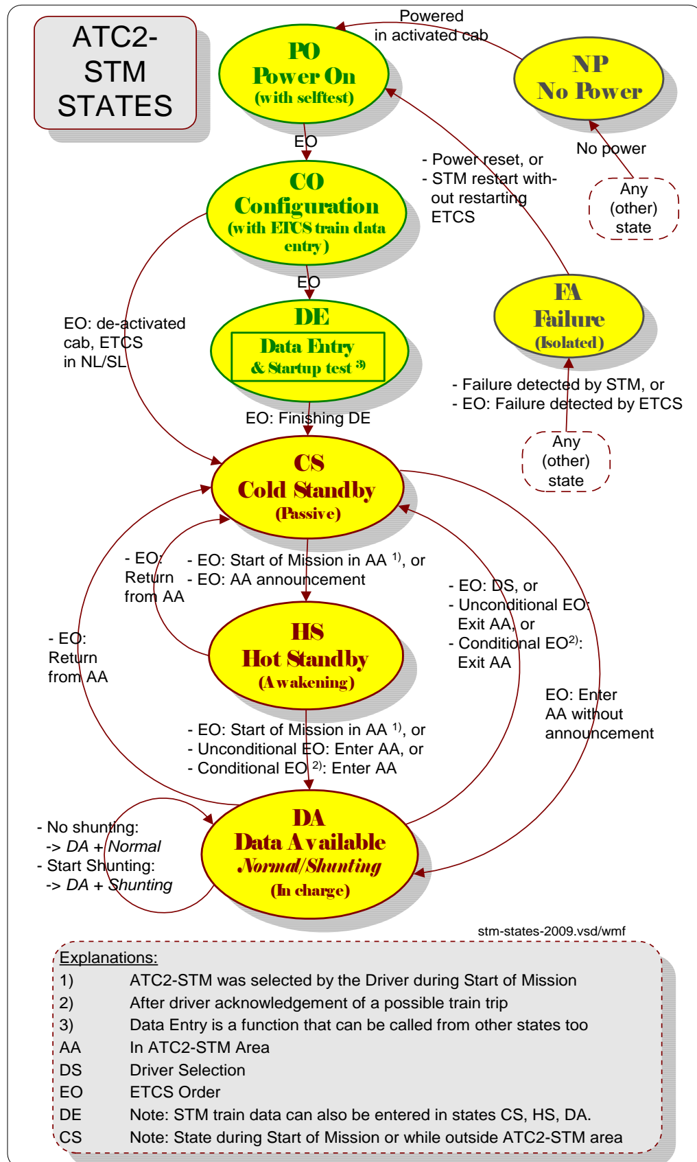
Figure 4.3-1. Note. STM State Transitions
