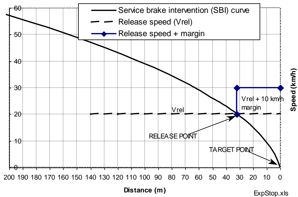
DISTANT SIGNAL BRAKING CURVE WITH "EXPECT STOP"
