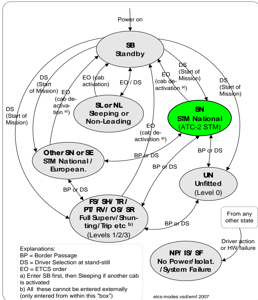
Figure 4.3-2. ETCS Mode & Level Transitions Overview
