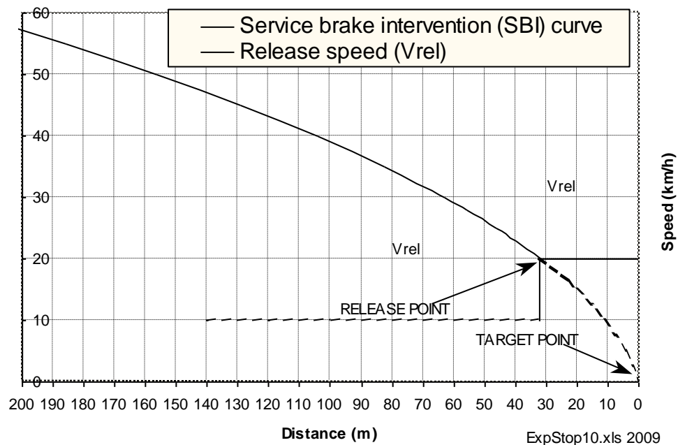
DISTANT SIGNAL BRAKING CURVE WITH "EXPECT STOP"
