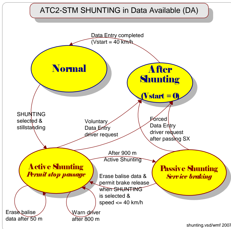
Figure 4.3-3. Shunting state machine
