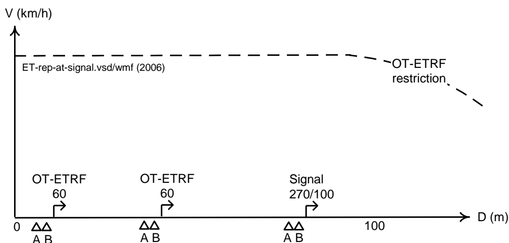
Figure 4.4-1. Repetition of OT-ET at the same signal
