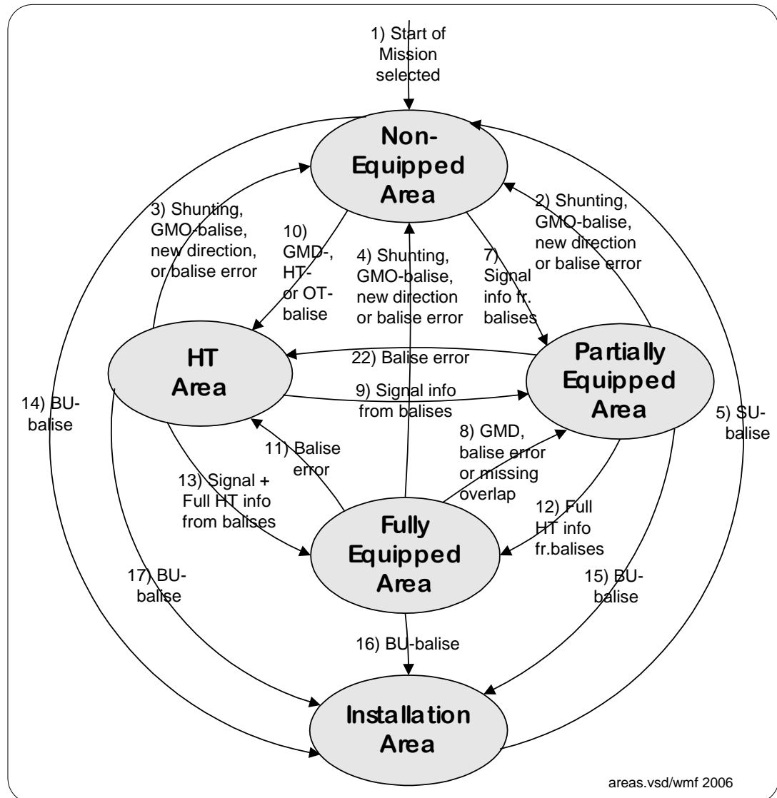
Figure 4.4-1. Area transitions
