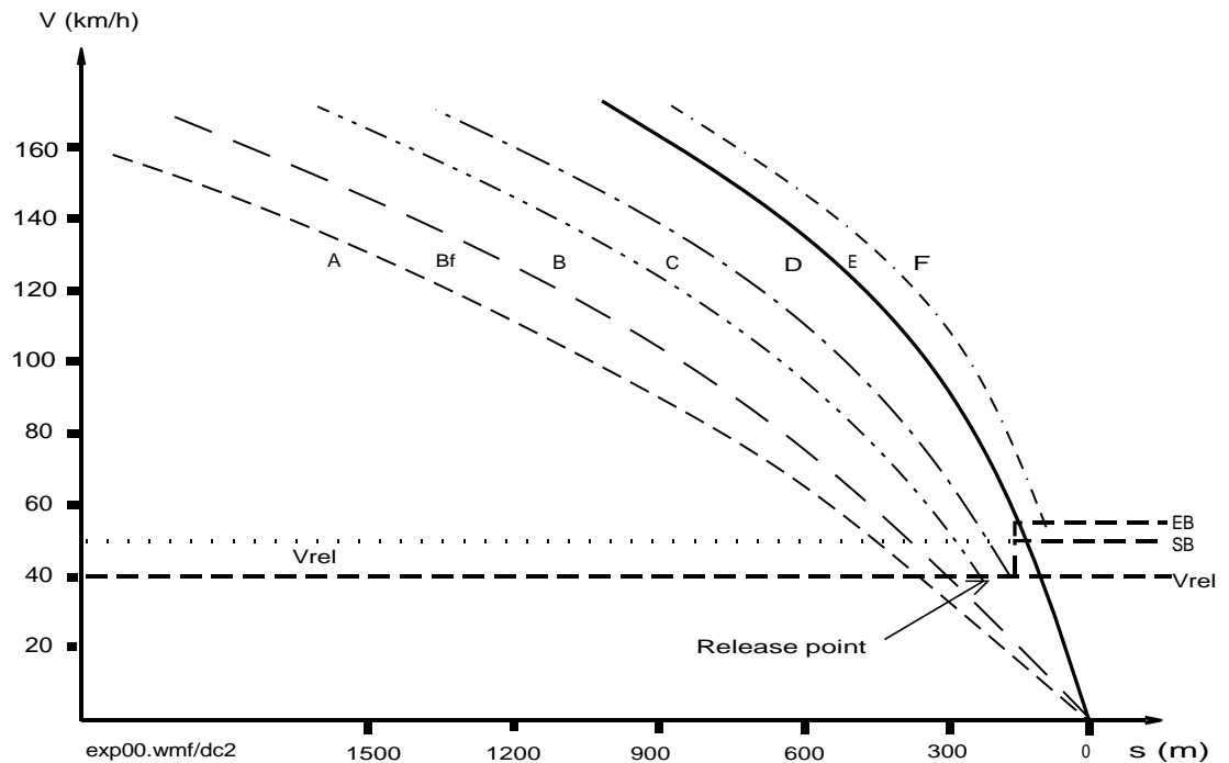
Figure 4.9-2. The position of the release point at 40-supervision
