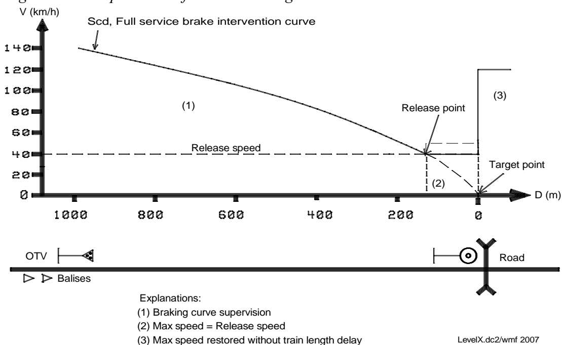
Figure 4.6-3. Supervision of a level crossing
